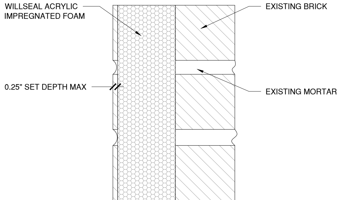
1 SECTION VIEW
