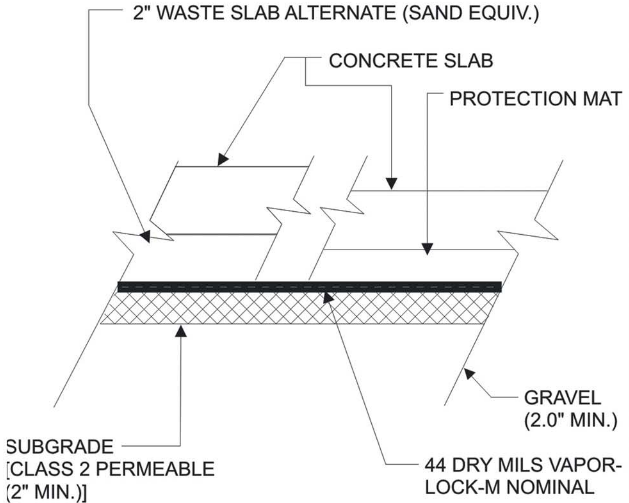
TYPICAL VAPOR BARRIER UNDER SLAB
