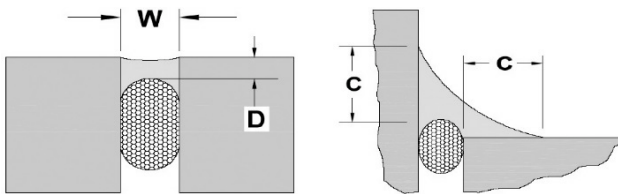
Figure 1 sealant bead width and depth recommendations and appropriate joint design
