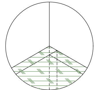
DETAIL B INSIDE CORNER BUTT JOINT
