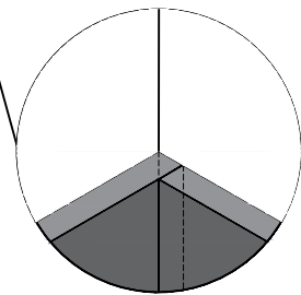
Option 1 Butt joint - inside corner
