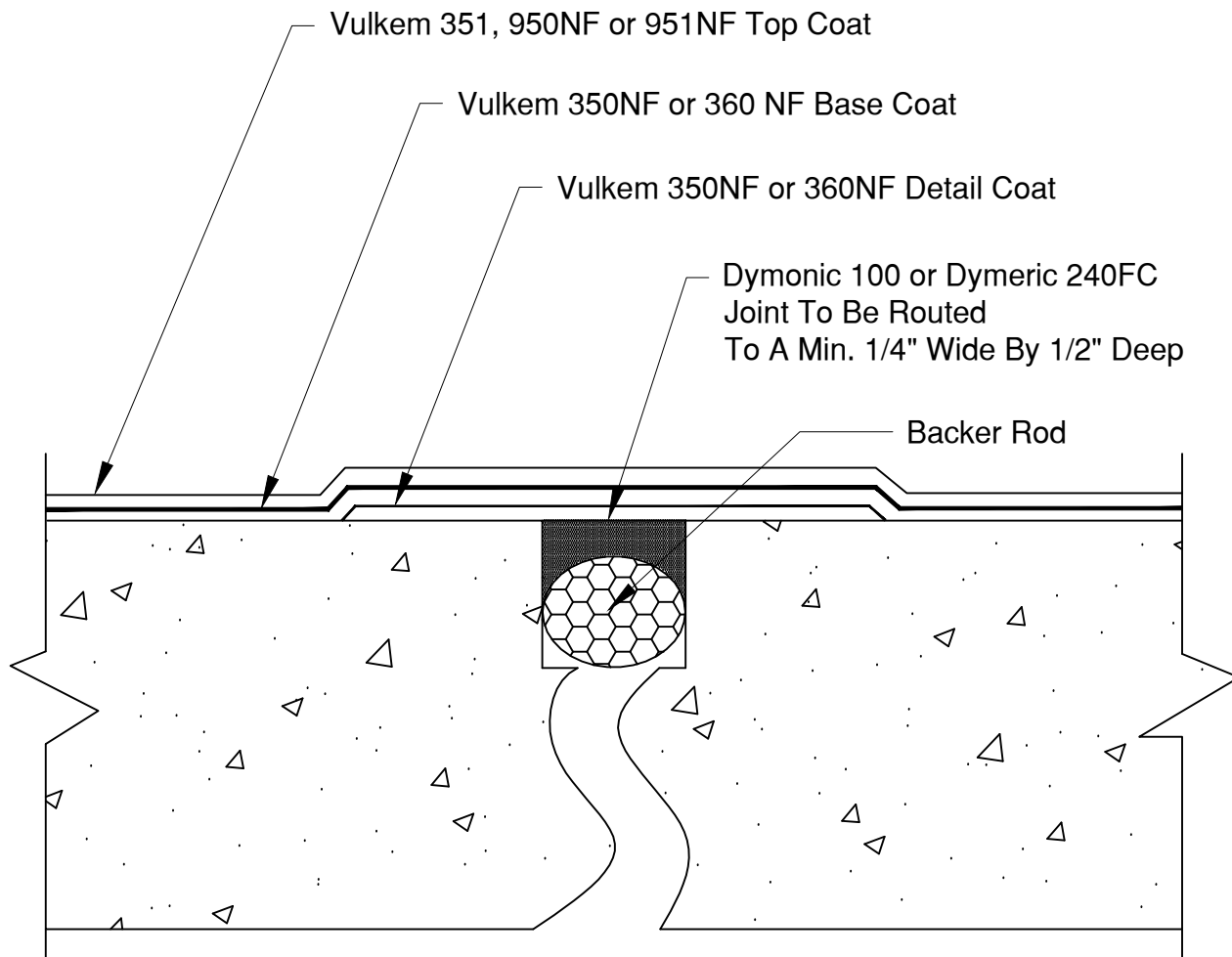
Treatment Of Cracks Greater Than 1/16"
