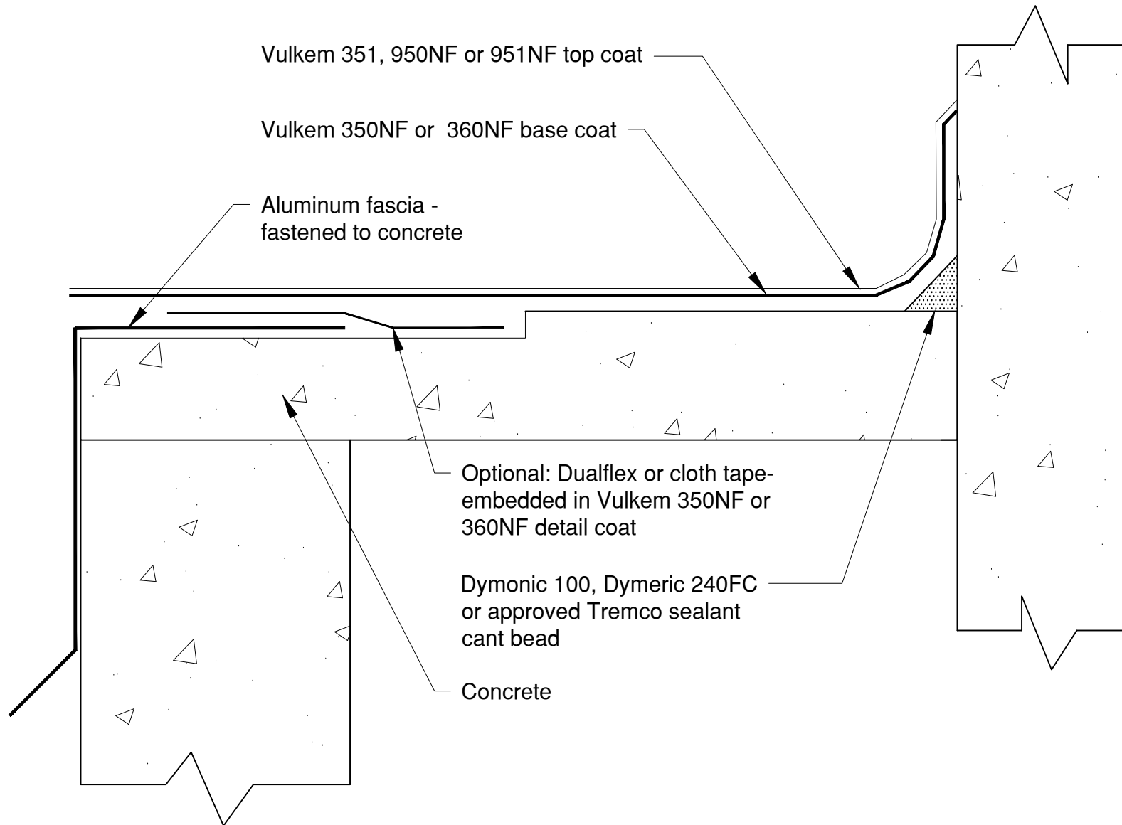
Typical Edge Detail On Concrete
